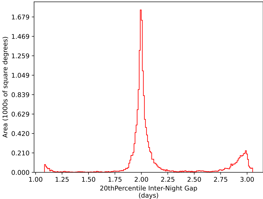
weather_cloudso36v3.4_10yrs WFD i band: 20thPercentile Inter-Night Gap
