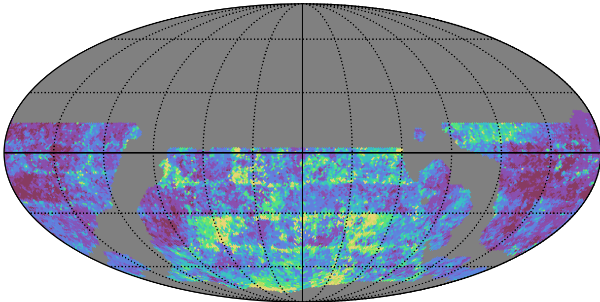
weather_cloudso36v3.4_10yrs WFD g band: 20thPercentile Inter-Night Gap
