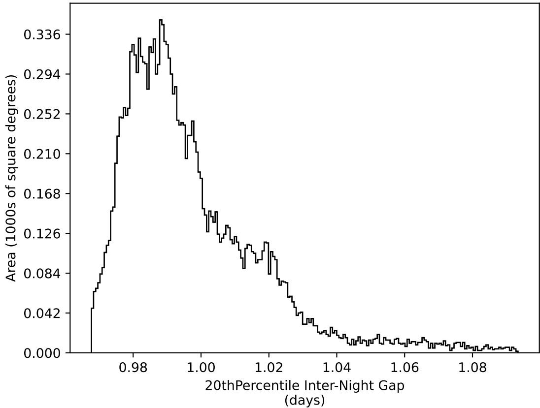
weather_cloudso36v3.4_10yrs WFD all bands: 20thPercentile Inter-Night Gap
