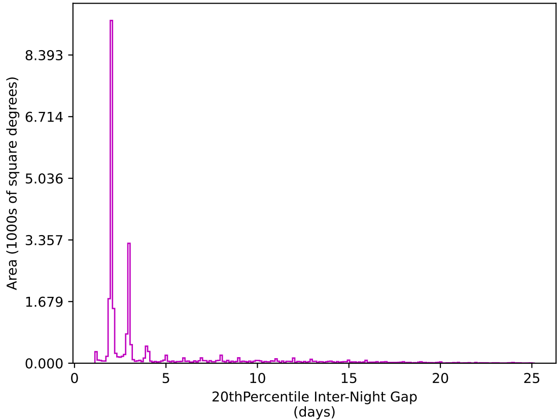
weather_cloudso36v3.4_10yrs All sky z band: 20thPercentile Inter-Night Gap
