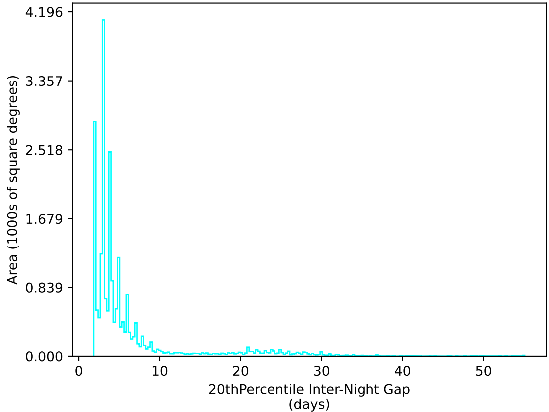
weather_cloudso36v3.4_10yrs All sky u band: 20thPercentile Inter-Night Gap
