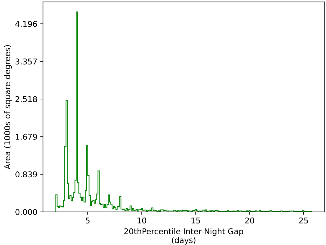
weather_cloudso36v3.4_10yrs All sky g band: 20thPercentile Inter-Night Gap
