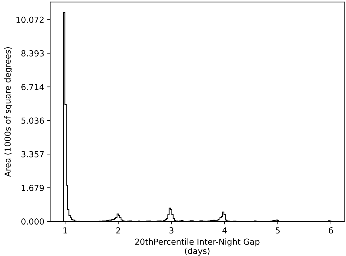
weather_cloudso36v3.4_10yrs All sky all bands: 20thPercentile Inter-Night Gap
