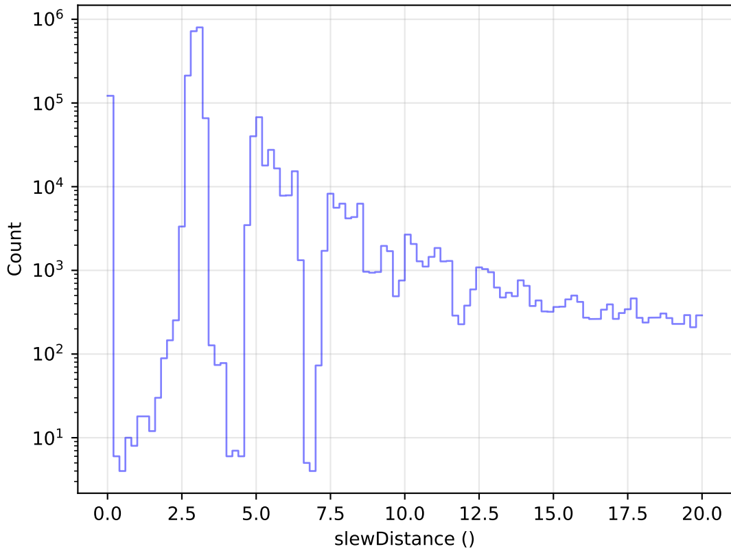
weather_cloudso36v3.4_10yrs All visits: Zoom Slew Distance Histogram
