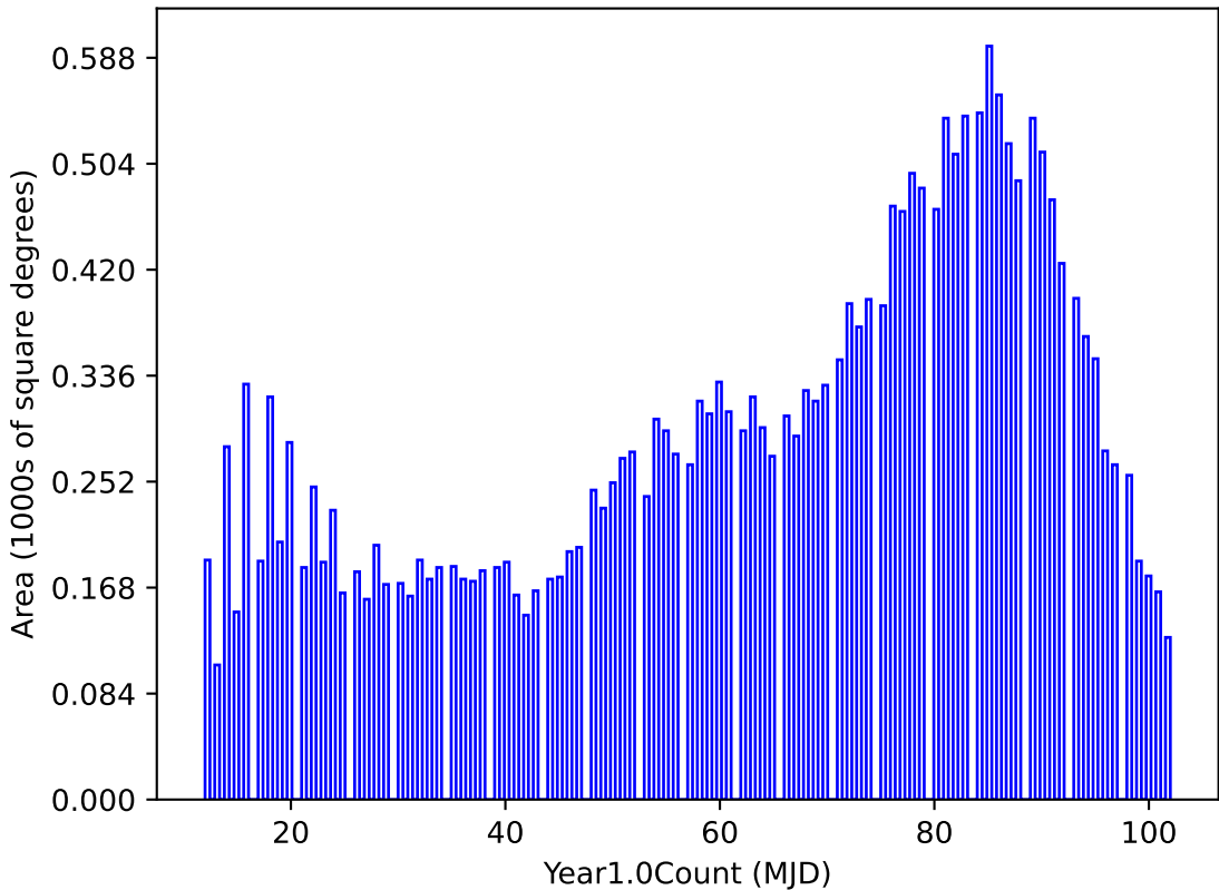
weather_cloudso36v3.4_10yrs night < 365.25: Year1.0Count
