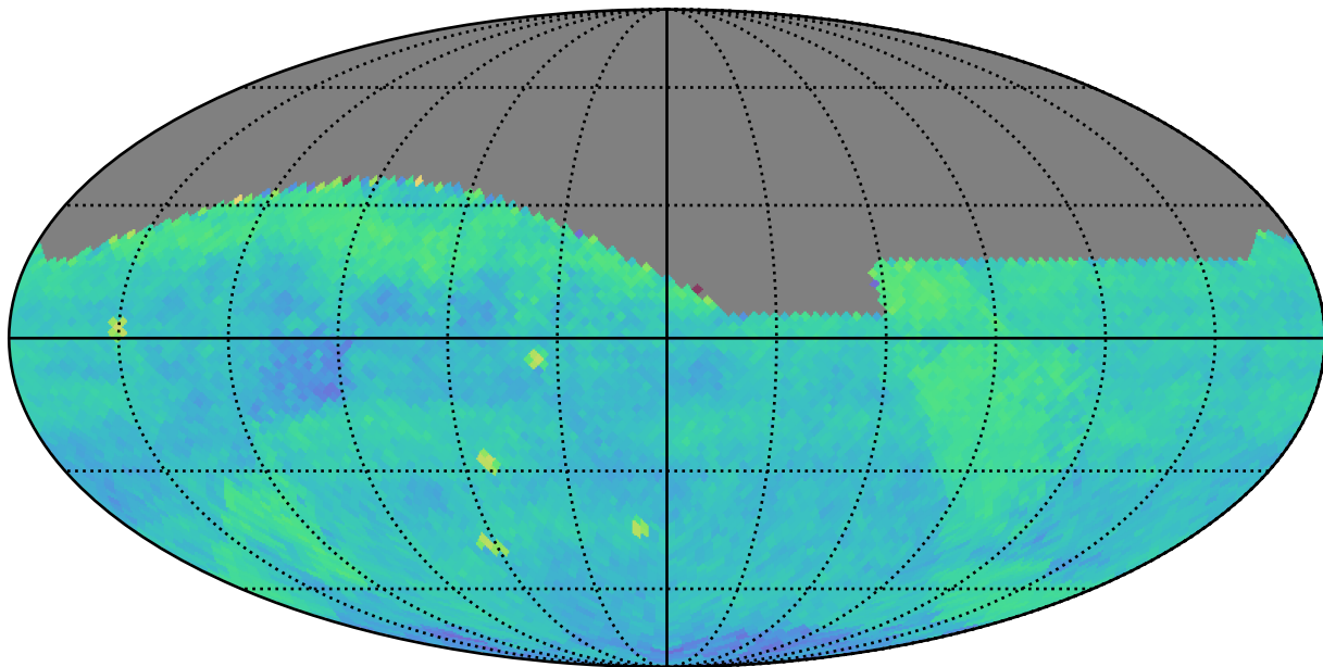
weather_cloudso36v3.4_10yrs (g or r or i): PairFraction
