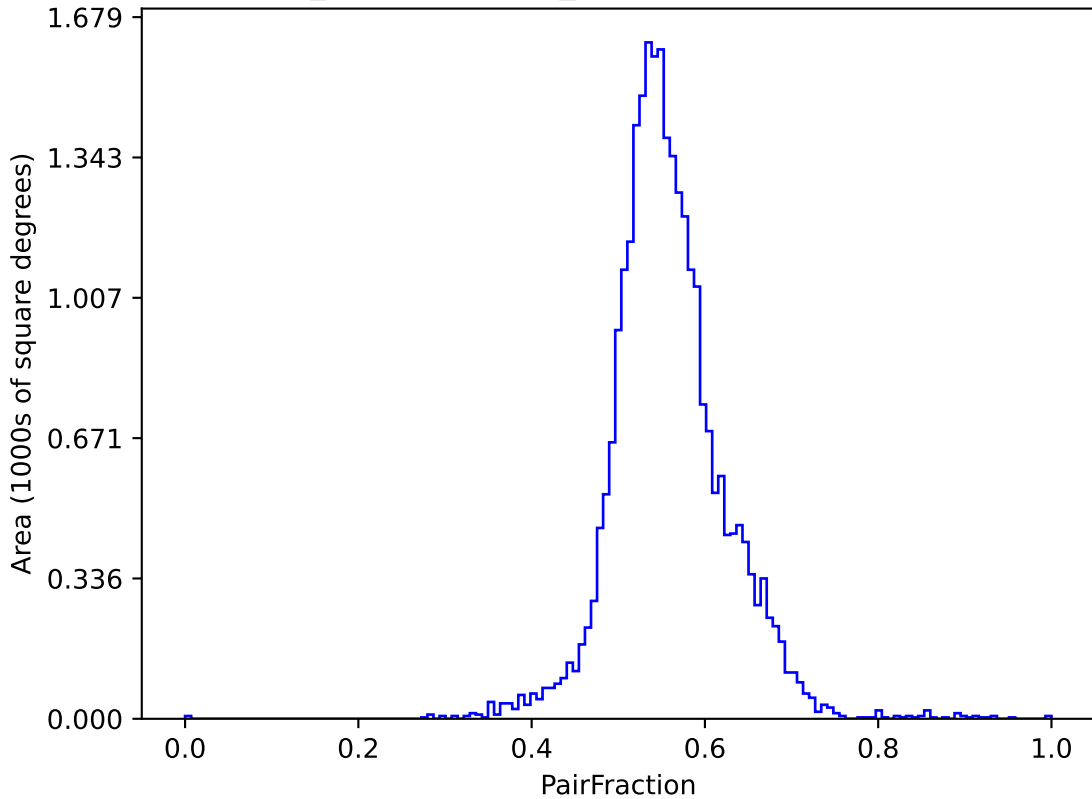
weather_cloudso36v3.4_10yrs (g or r or i): PairFraction
