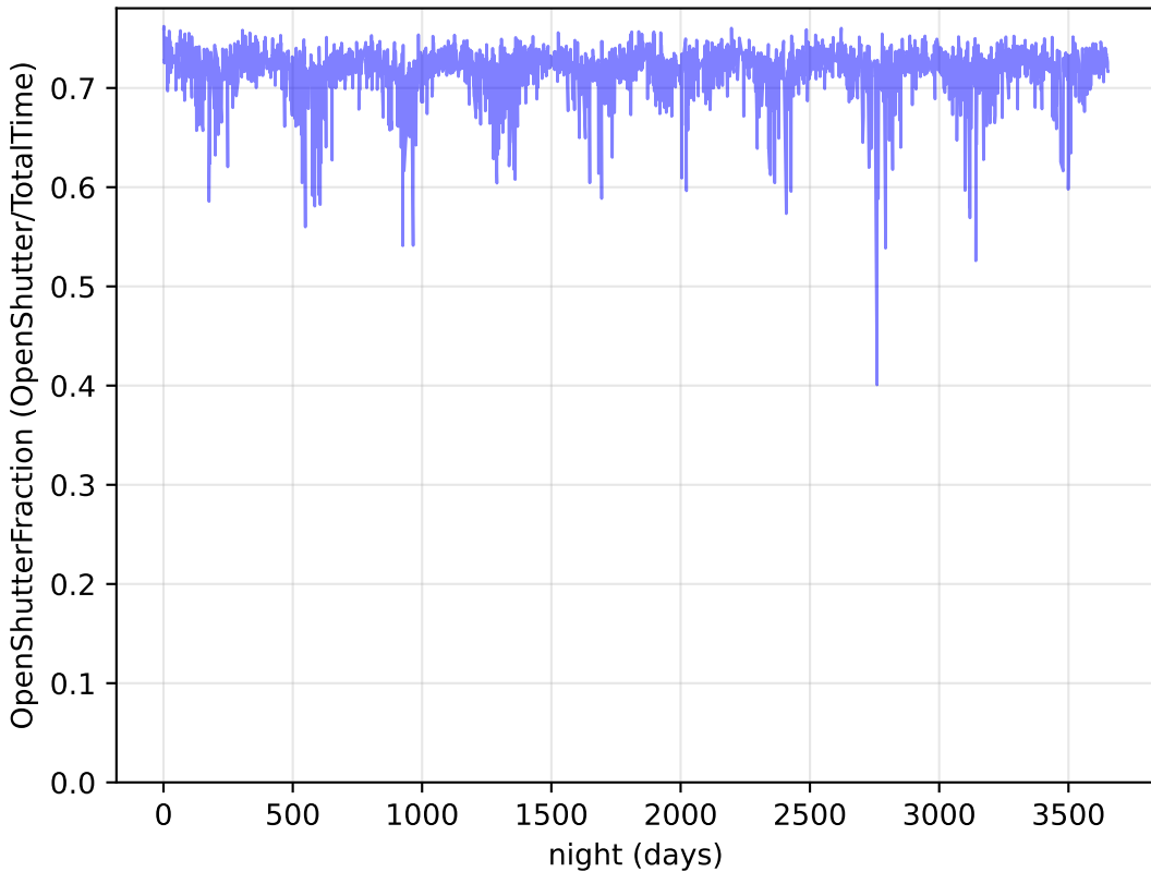
weather_cloudso36v3.4_10yrs : OpenShutterFraction
