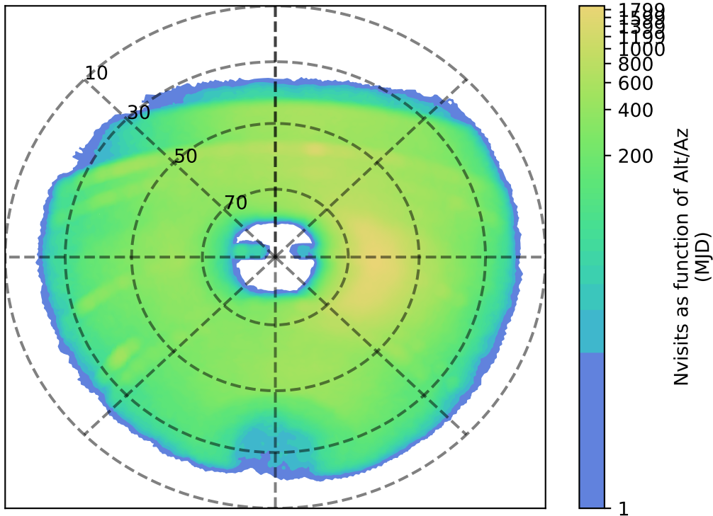
weather_cloudso36v3.4_10yrs y: Nvisits as function of Alt/Az
