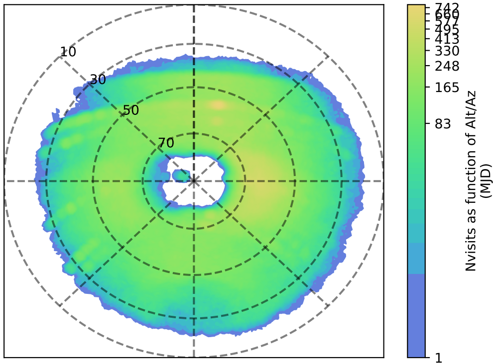
weather_cloudso36v3.4_10yrs u: Nvisits as function of Alt/Az
