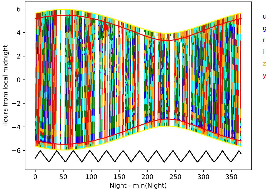
weather_cloudso36v3.4_10yrs year 3-4: Hourglass
