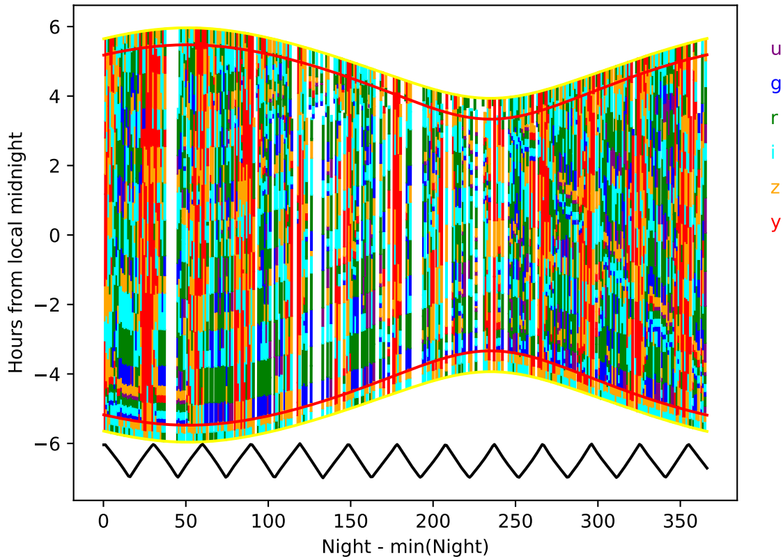
weather_cloudso36v3.4_10yrs year 1-2: Hourglass
