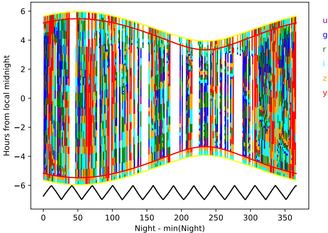
weather_cloudso36v3.4_10yrs year 0-1: Hourglass
