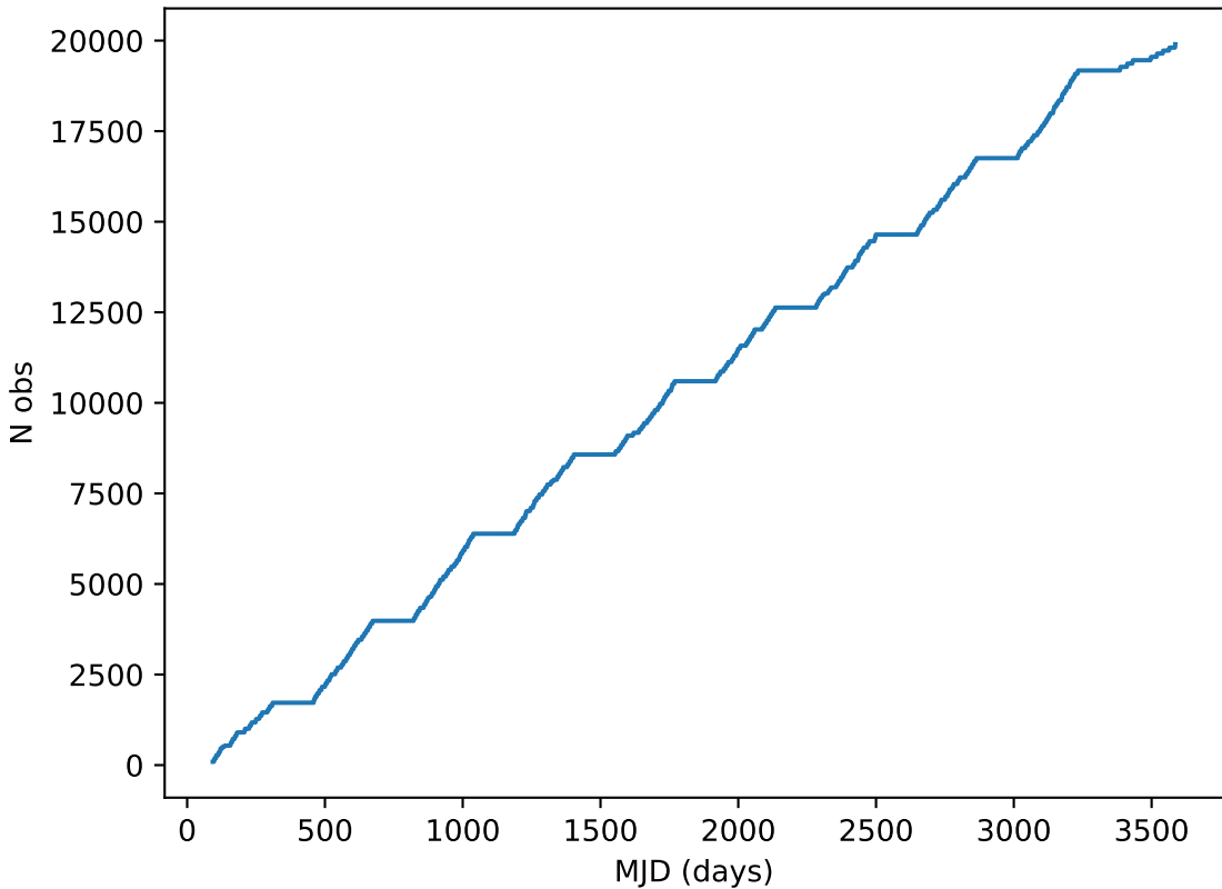
weather_cloudso36v3.4_10yrs note like DD:ECDFS%: Cumulative
