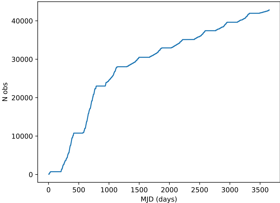
weather_cloudso36v3.4_10yrs note like DD:COSMOS%: Cumulative
