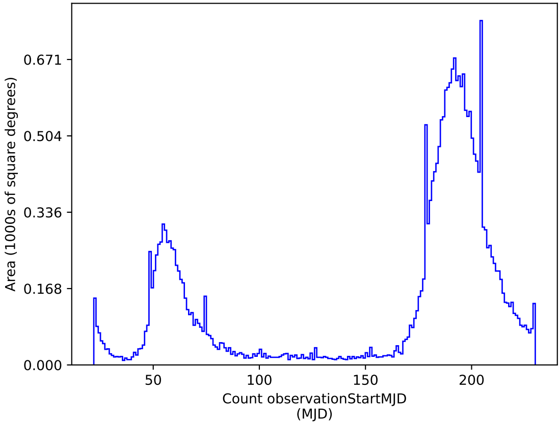
weather_cloudso36v3.4_10yrs r: Count observationStartMJD
