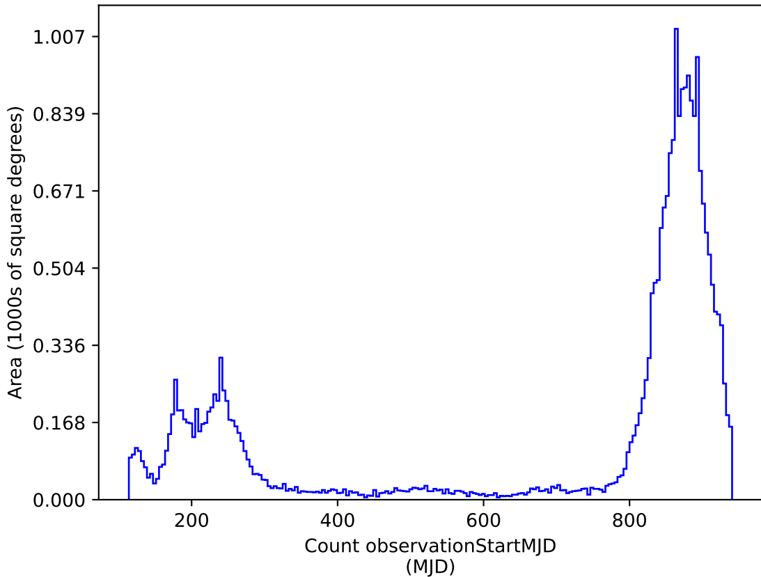
weather_cloudso36v3.4_10yrs : Count observationStartMJD
