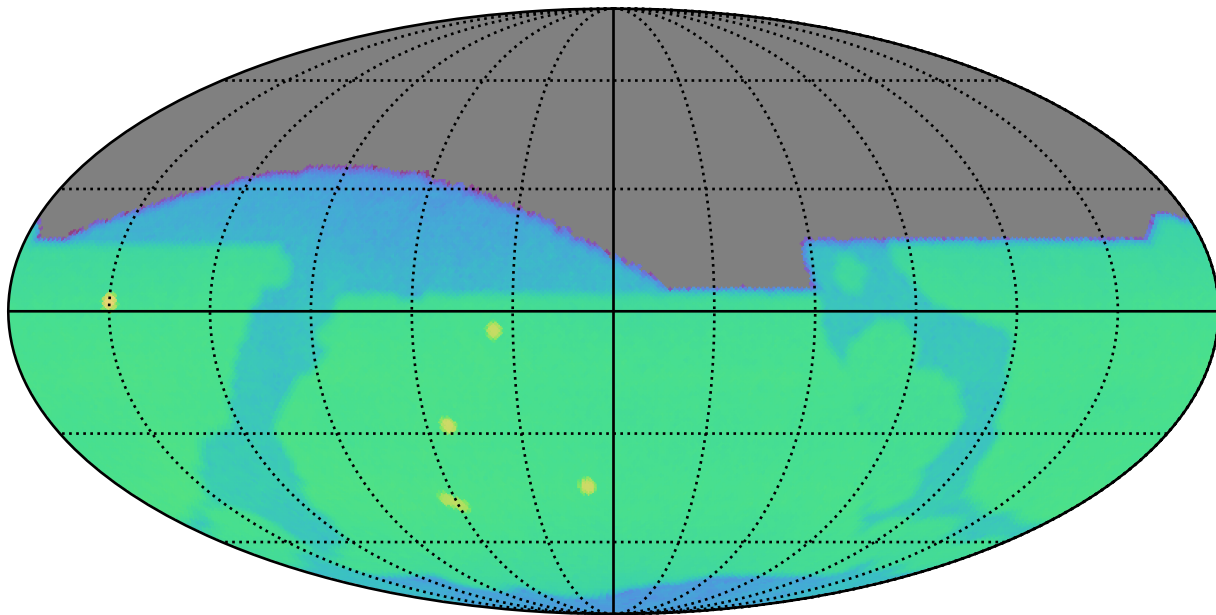
weather_cloudso36v3.4_10yrs z: CoaddM5
