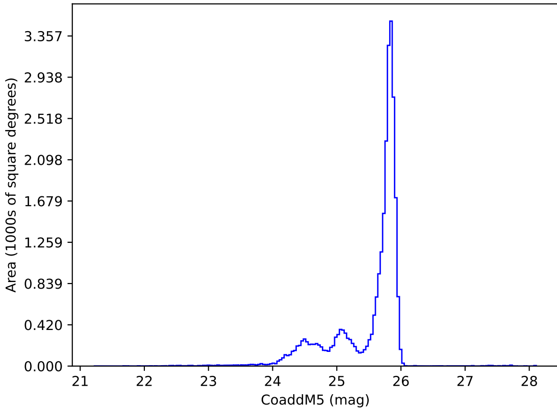
weather_cloudso36v3.4_10yrs z: CoaddM5
