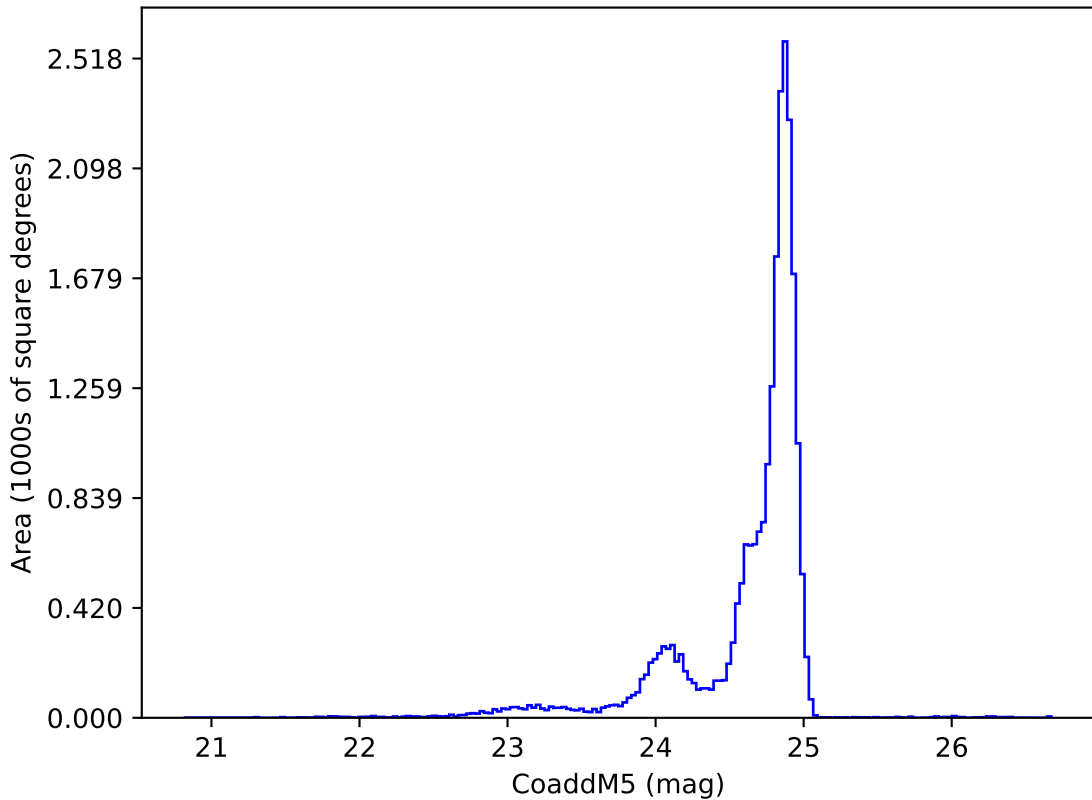
weather_cloudso36v3.4_10yrs y: CoaddM5
