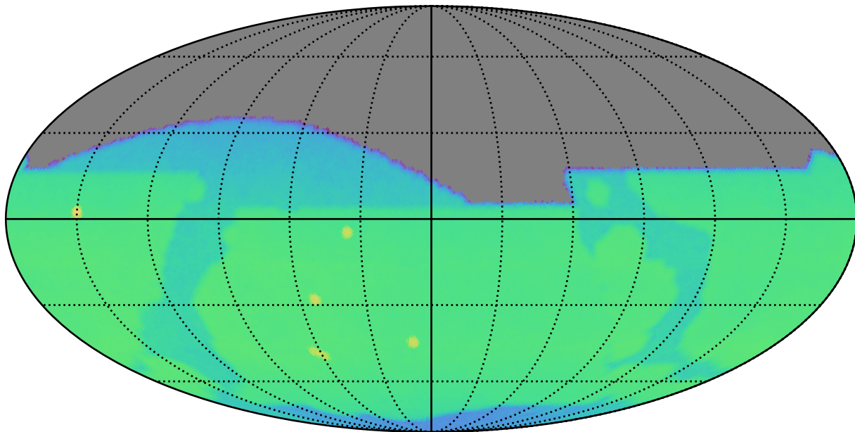
weather_cloudso36v3.4_10yrs r: CoaddM5
