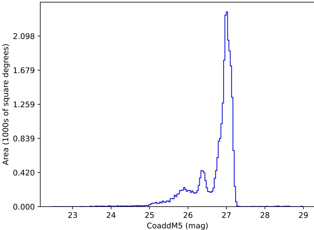
weather_cloudso36v3.4_10yrs r: CoaddM5
