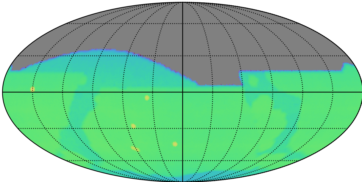
weather_cloudso36v3.4_10yrs : CoaddM5
