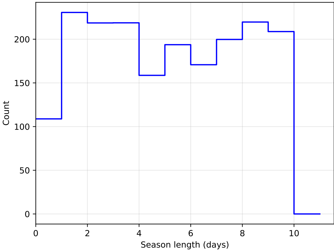
weather_cloudso36v3.4_10yrs DD:WFD all bands: SeasonLength
