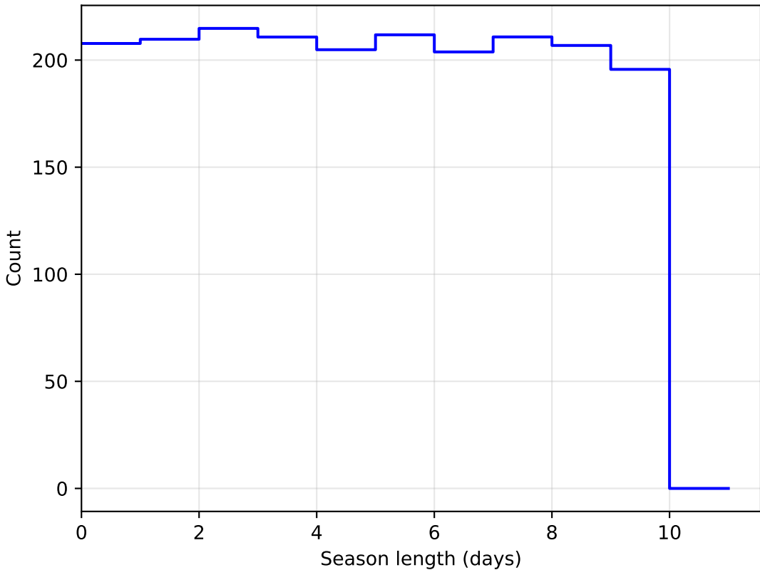
weather_cloudso36v3.4_10yrs DD:EDFS all bands: SeasonLength
