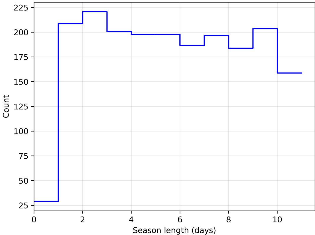
weather_cloudso36v3.4_10yrs DD: COSMOS all bands: SeasonLength
