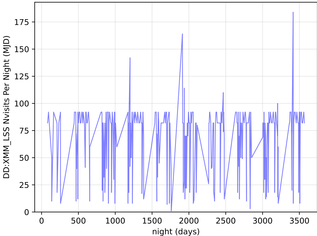
weather_cloudso36v3.4_10yrs all bands: DD:XMM_LSS Nvisits Per Night
