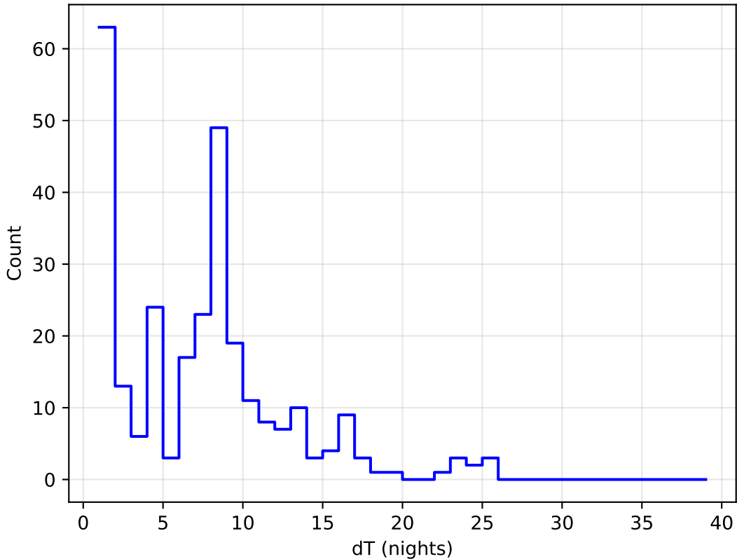
weather_cloudso36v3.4_10yrs all bands: DD:XMM_LSS Delta Nights Histogram
