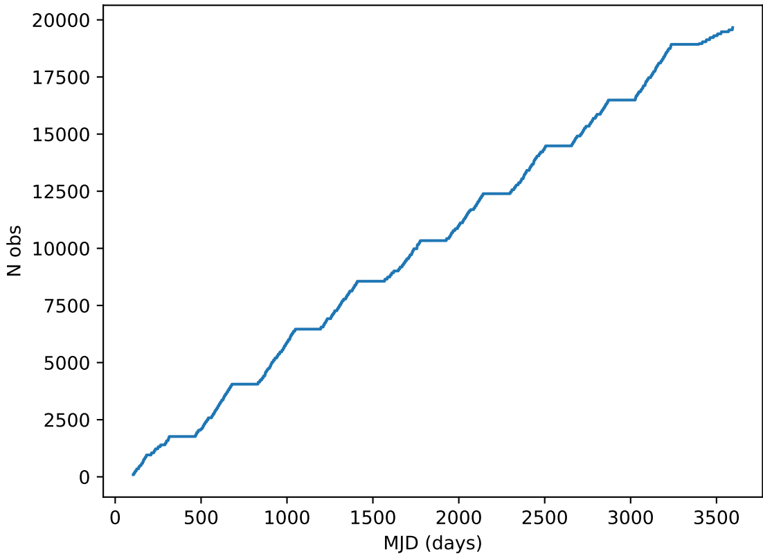
weather_cloudso36v3.4_10yrs all bands: DD:EDFS Cumulative NVisits
