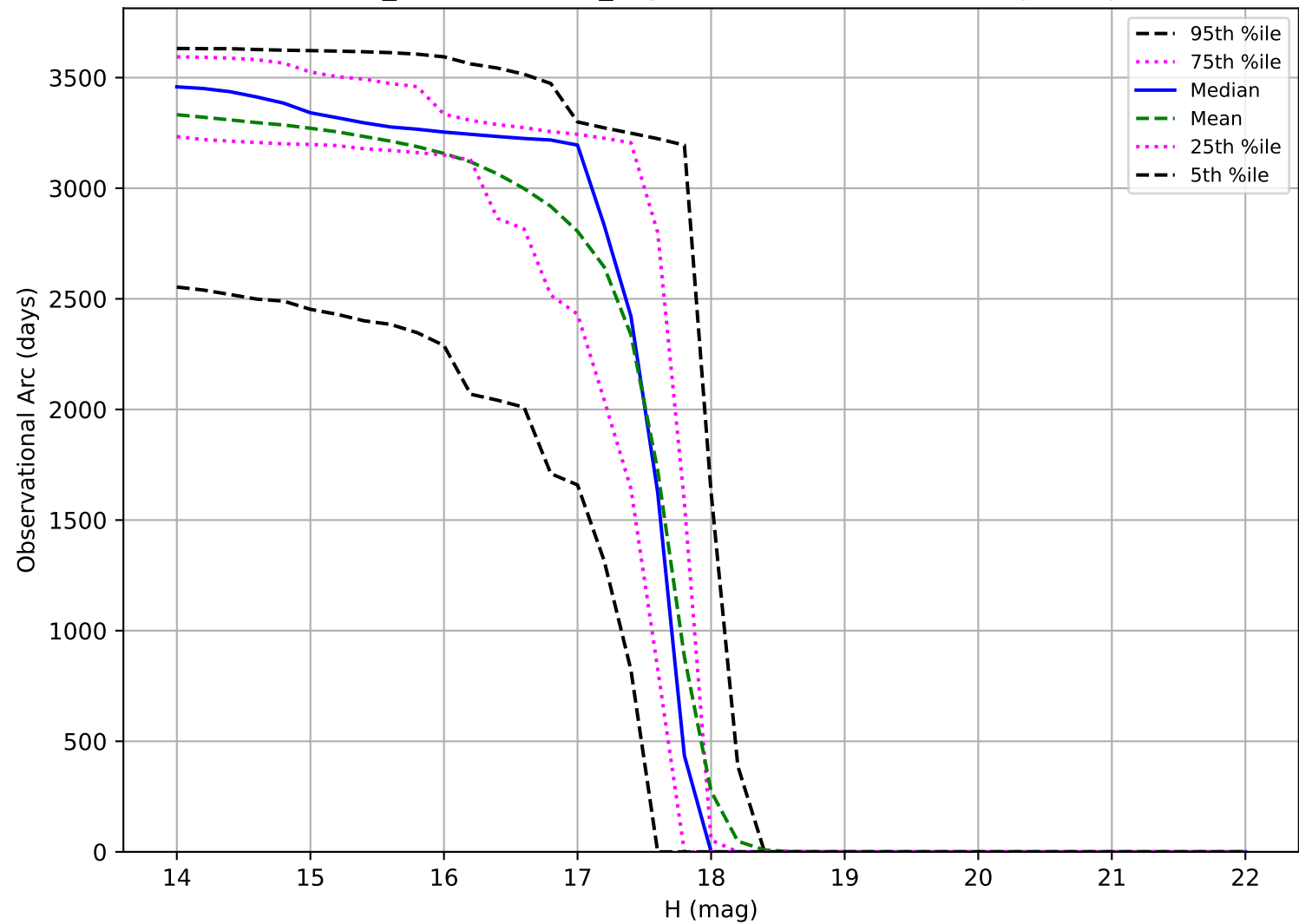
weather_cloudso35v3.4_10yrs: Observational Arc Length Trojan
