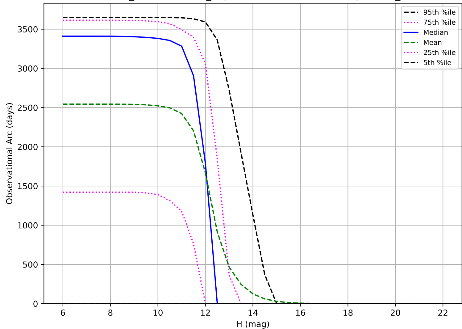
weather_cloudso35v3.4_10yrs: Observational Arc Length OCC_r20
