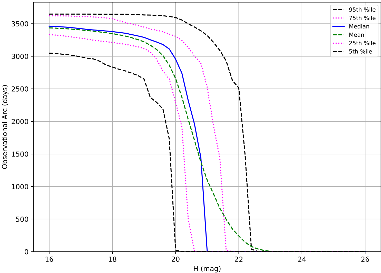
weather_cloudso35v3.4_10yrs: Observational Arc Length MBA
