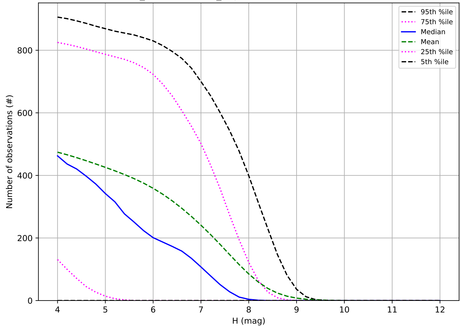
weather_cloudso35v3.4_10yrs: Number of observations TNO
