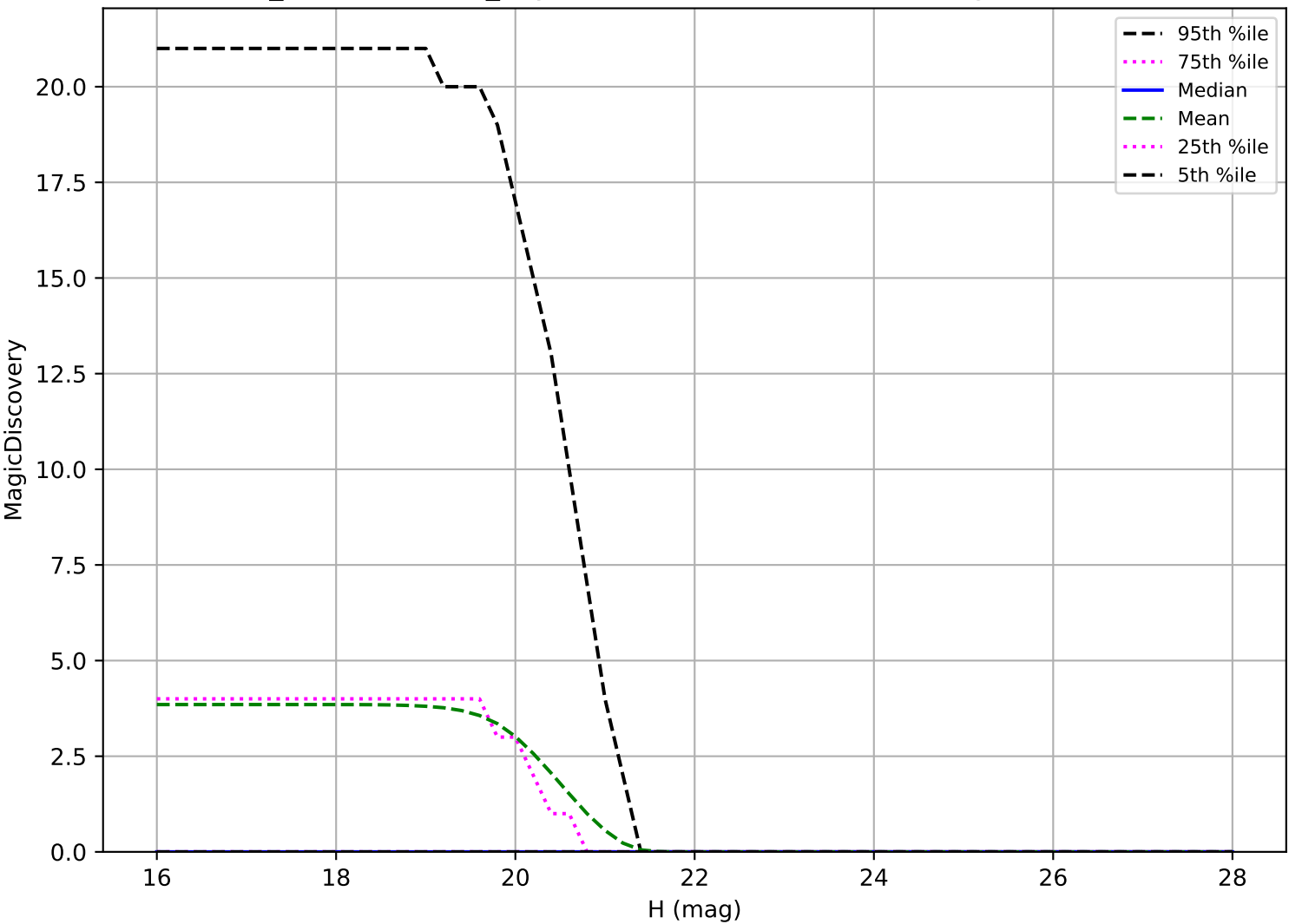
weather_cloudso35v3.4_10yrs: Vatira 6 detections in 60 nights detection loss
