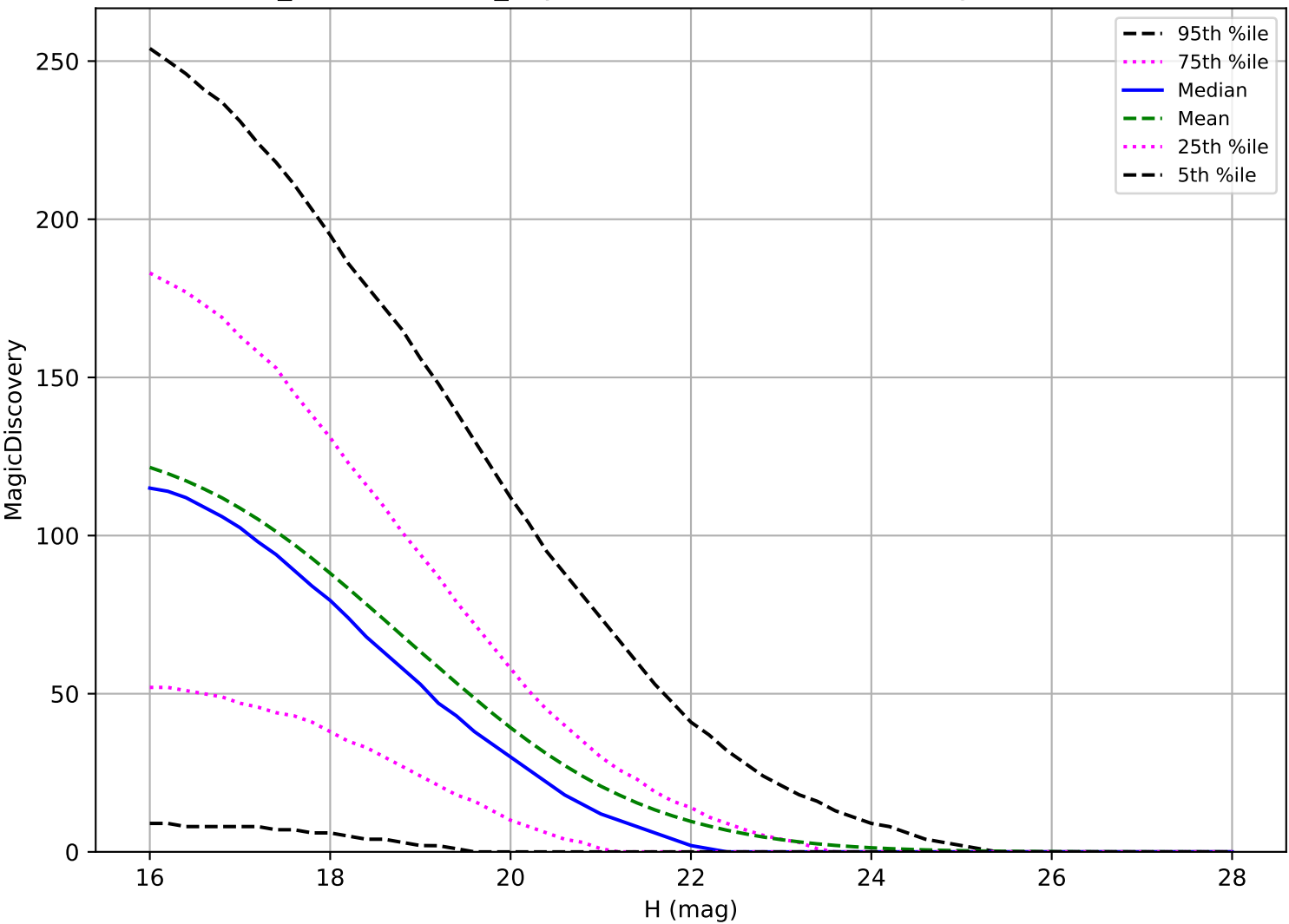
weather_cloudso35v3.4_10yrs: PHA 6 detections in 60 nights detection loss
