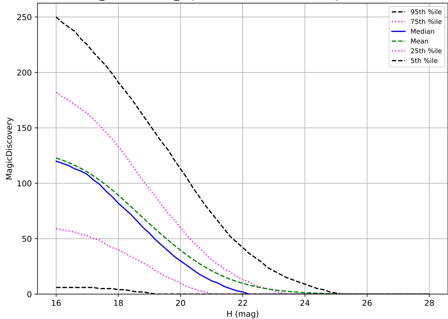
weather_cloudso35v3.4_10yrs: NEO 6 detections in 60 nights detection loss
