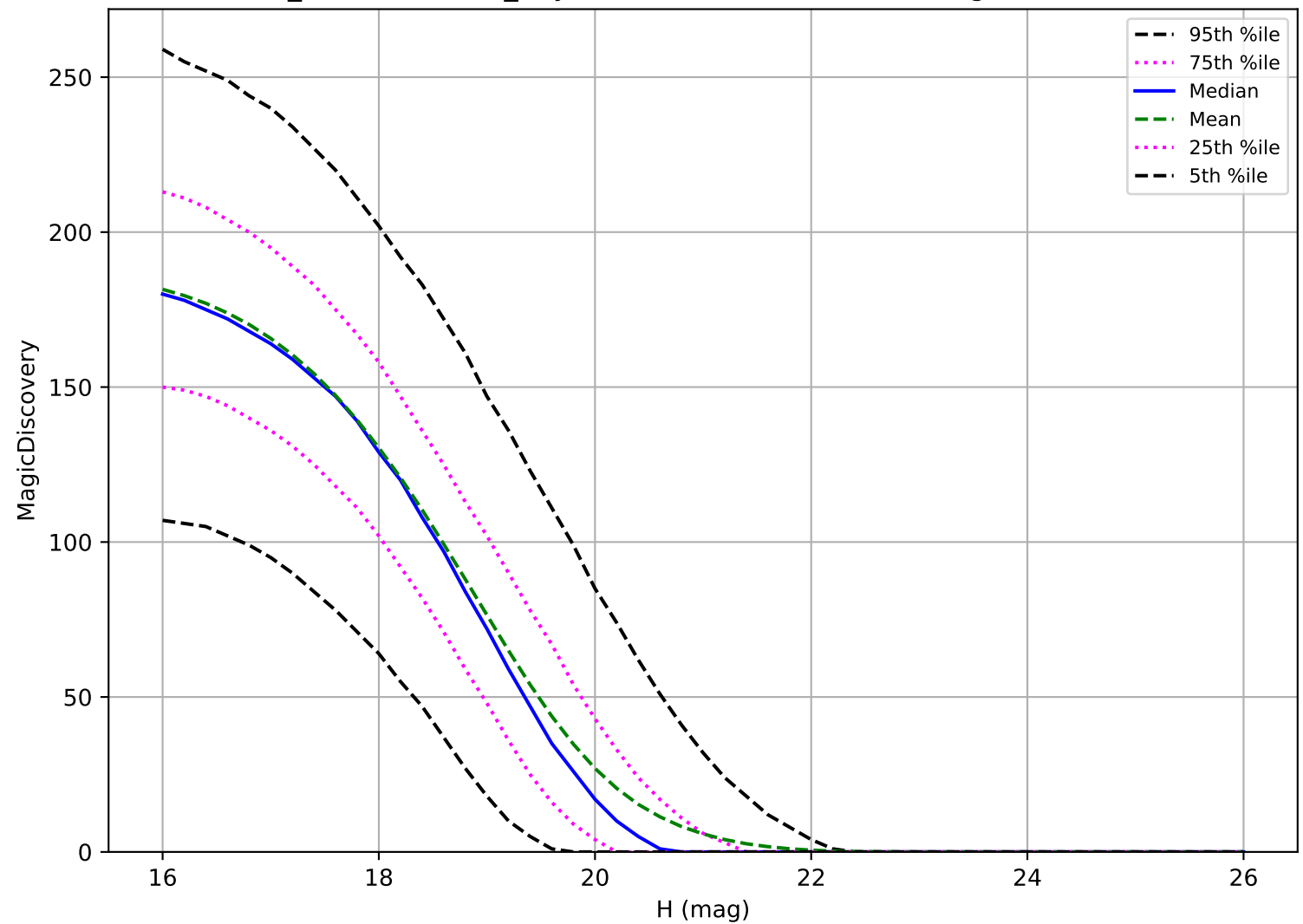
weather_cloudso35v3.4_10yrs: MBA 6 detections in 60 nights detection loss
