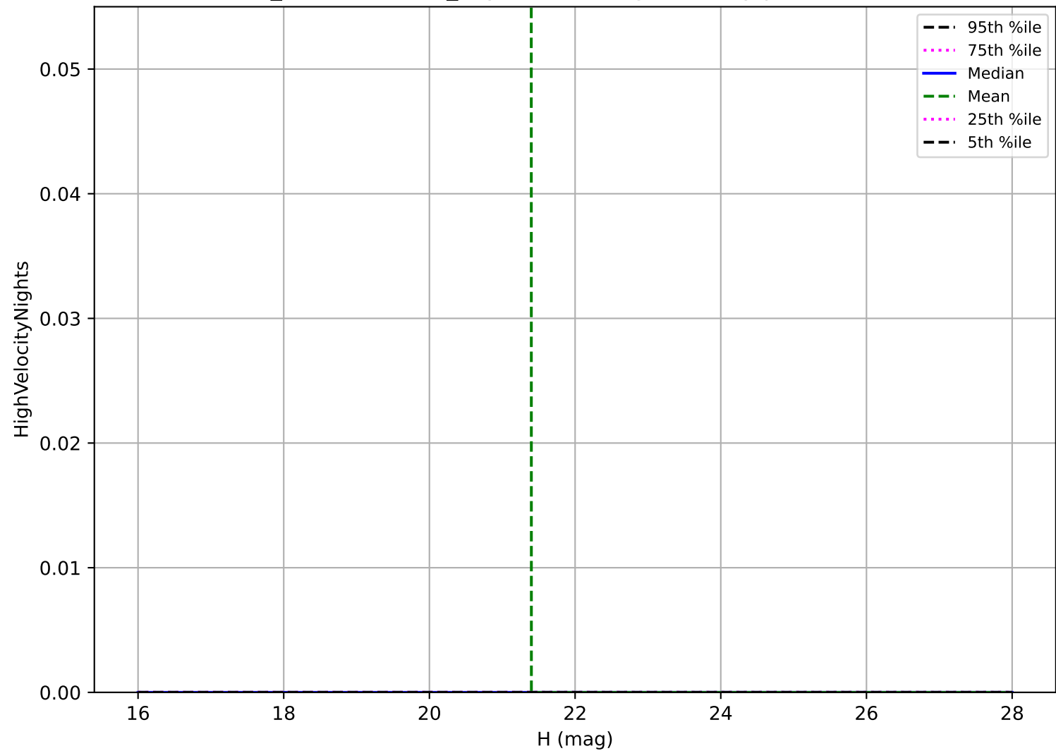
weather_cloudso35v3.4_10yrs: Vatira High velocity pair detection loss
