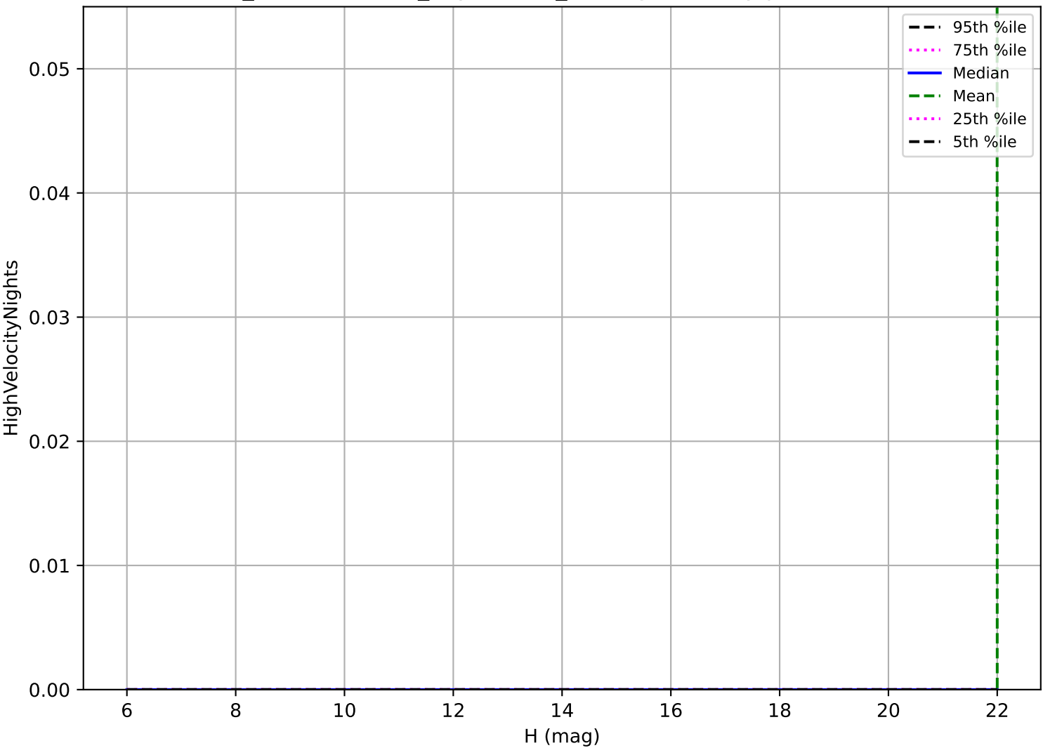
weather_cloudso35v3.4_10yrs: OCC_r20 High velocity pair detection loss
