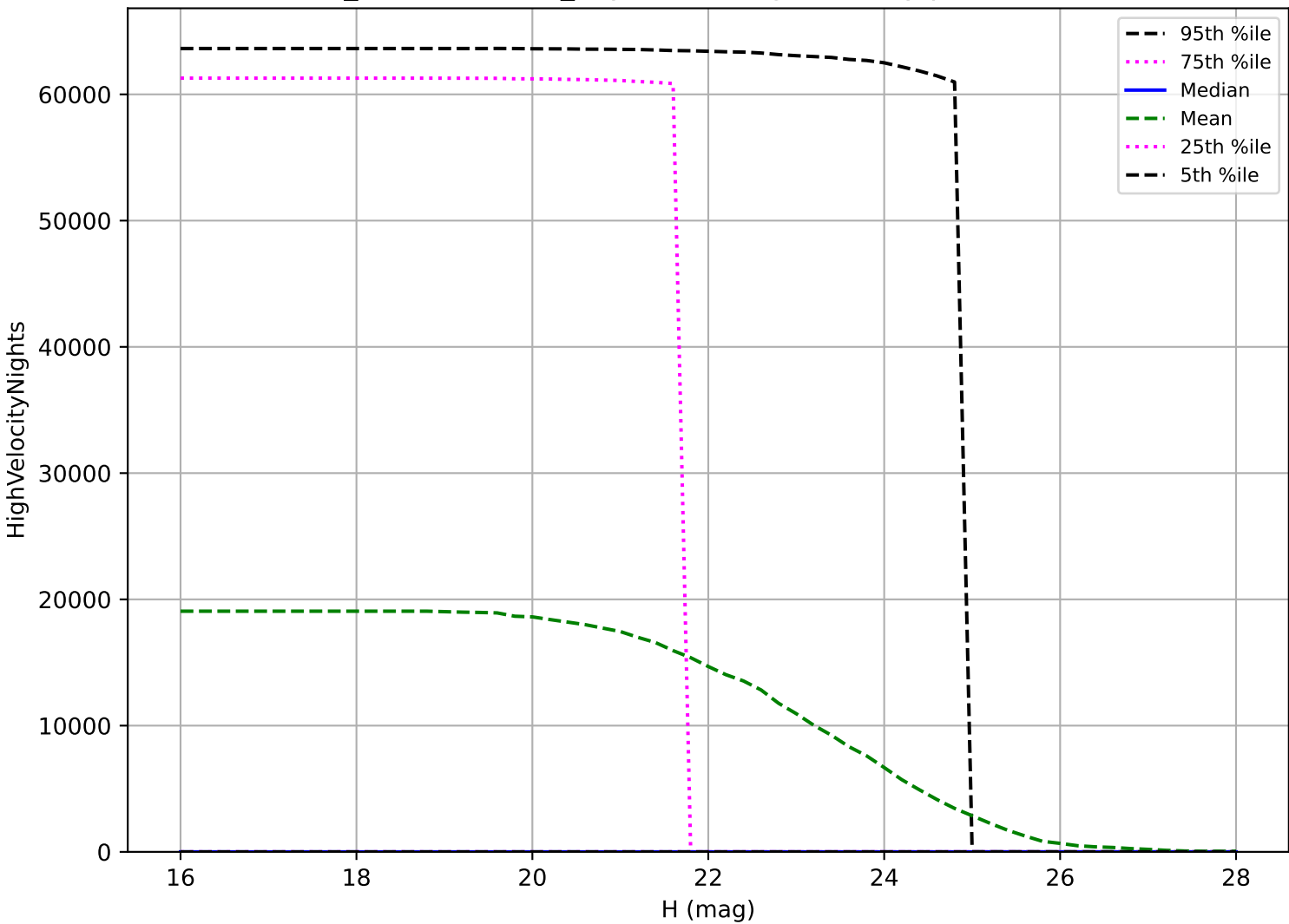
weather_cloudso35v3.4_10yrs: NEO High velocity pair detection loss
