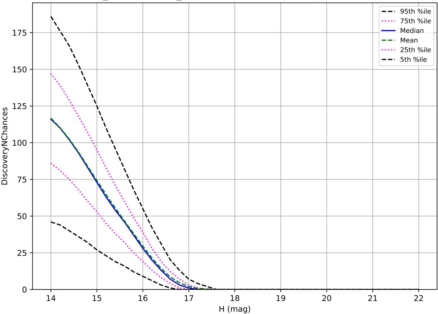
weather_cloudso35v3.4_10yrs: Trojan 3 pairs in 15 nights detection loss
