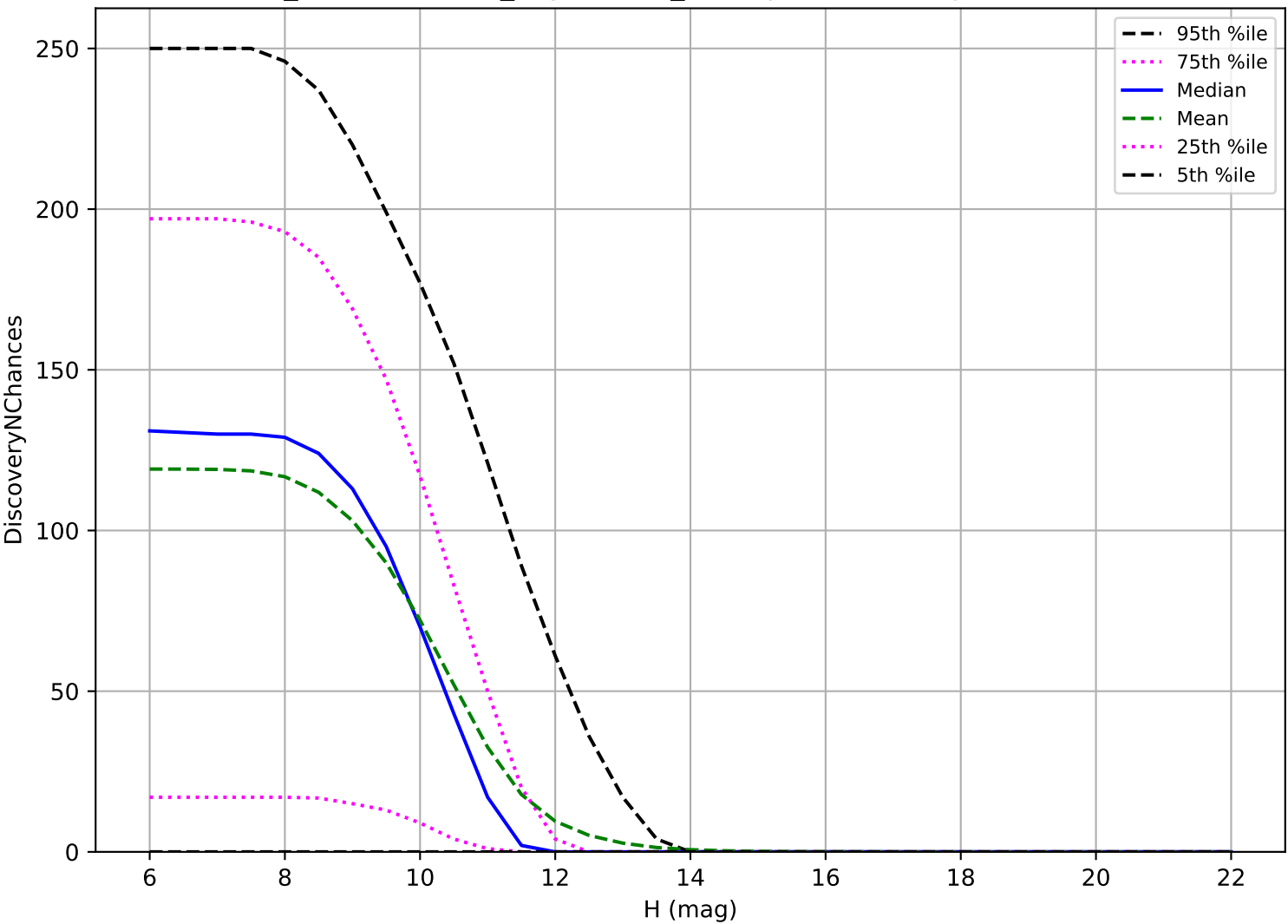
weather_cloudso35v3.4_10yrs: OCC_r20 3 pairs in 15 nights detection loss
