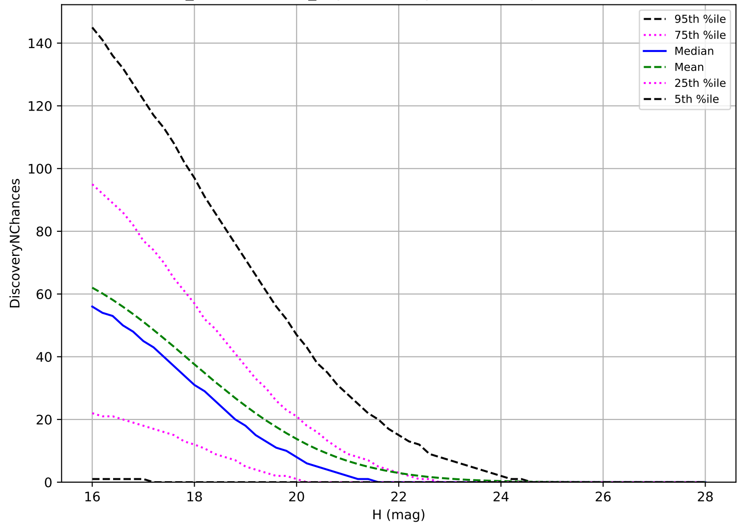
weather_cloudso35v3.4_10yrs: NEO 3 pairs in 15 nights detection loss
