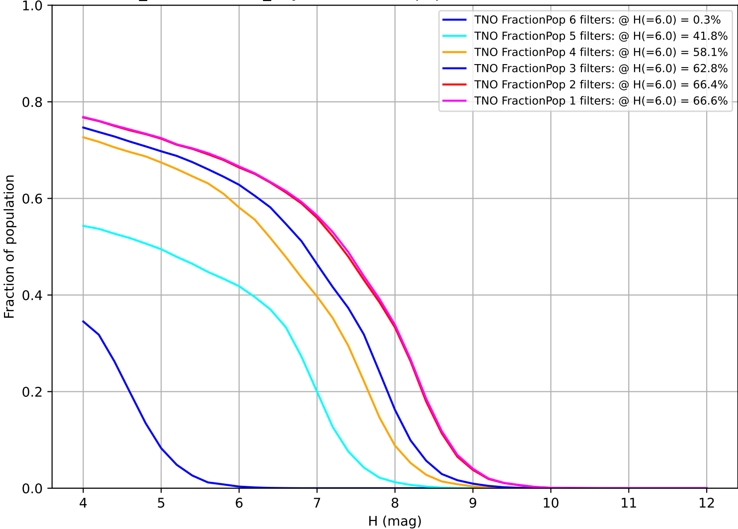
weather_cloudso35v3.4_10yrs: Fraction of population with colors in X filters TNO
