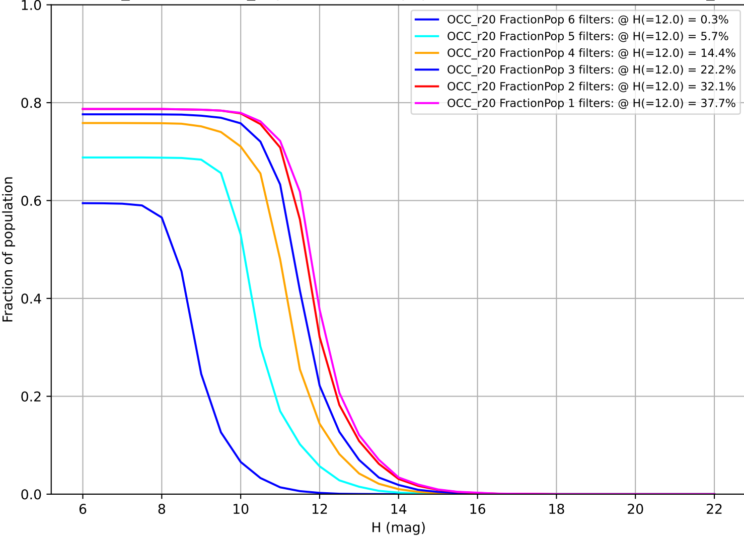
weather_cloudso35v3.4_10yrs: Fraction of population with colors in X filters OCC_r20
