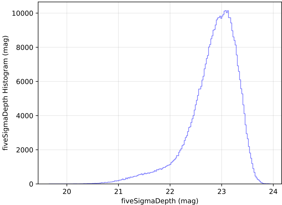
weather_cloudso35v3.4_10yrs z: fiveSigmaDepth Histogram
